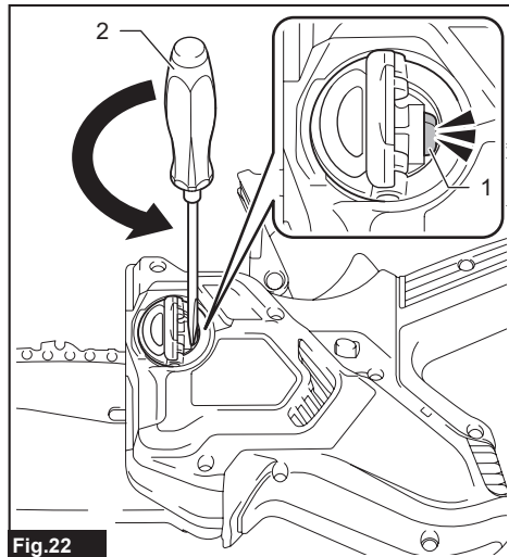
► 1. Slot 2. Slotted screwdriver
